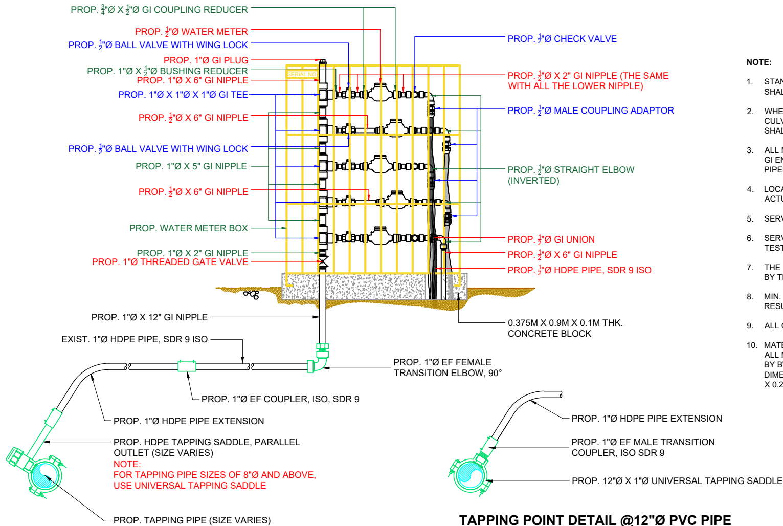
STANDARD STANDPIPE DETAIL
