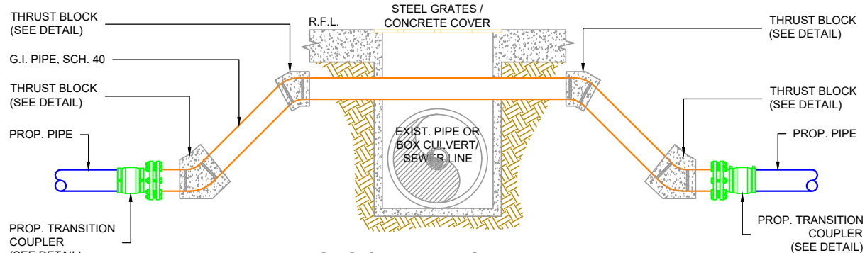
ALONG CULVERT / SEWER LINE
