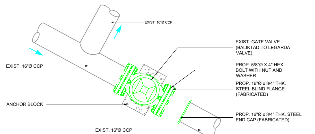
TIE-OUT POINT #1
